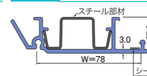
#78RW 既設管径:φ1000~1100
