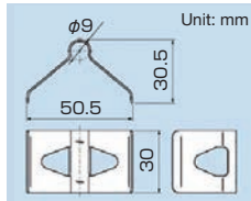
Continuous thread orthogonal brackets
