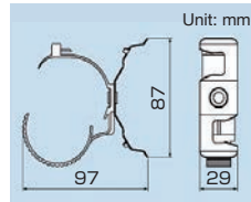
Piping support member
