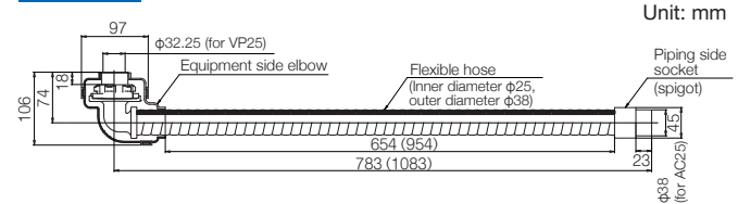
Spigot type
