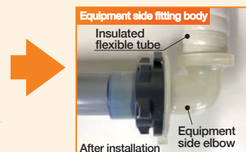
After installation
